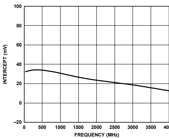
Figure 39. Intercept vs. Frequency, Supply 5 V
