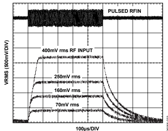
Figure 33. Output Response to Various RF Input Pulse Levels, Supply 3 V, Frequency 900 MHz, C_{FLTR} = \text{Open} , C_{OUT} = 0.1 \text{ uF} , R_{OUT} = 1 \text{ k}\Omega
