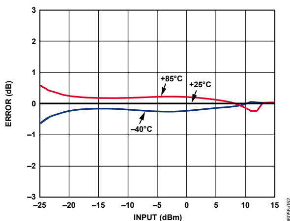
Figure 52. Error from +25^{\circ}\text{C} Output Voltage at -40^{\circ}\text{C} , +25^{\circ}\text{C} , and +85^{\circ}\text{C} After Ambient Normalization, Frequency 1900 MHz, Supply 5.0 V
